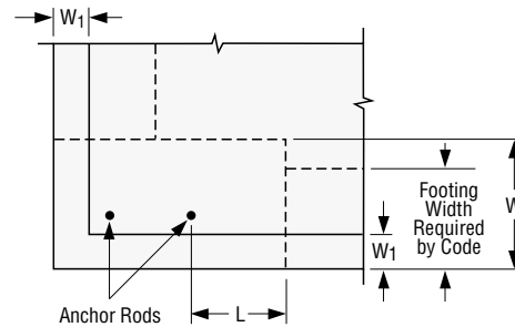
Plan View – Corner Installation Additional Adhesive Application
