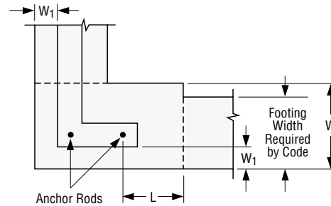
Plan View – Garage Front Additional Adhesive Application
