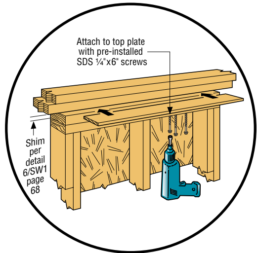
TOP-OF-WALL CONNECTION
