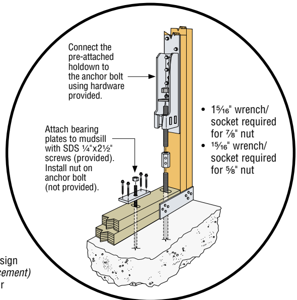
BOTTOM-OF-WALL INSTALLATION
